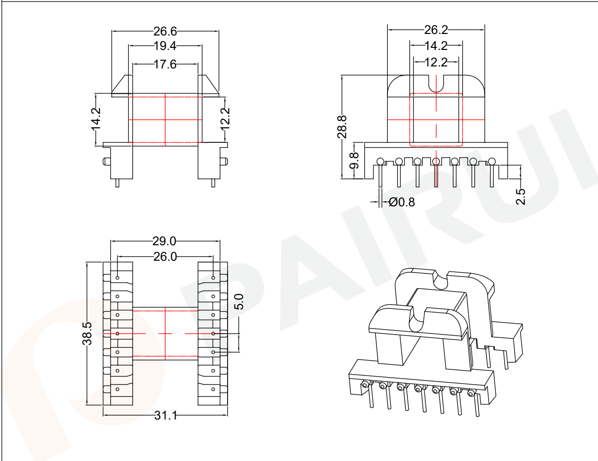
Winding data and area product for 14-pins EE40/17/11 coil former
