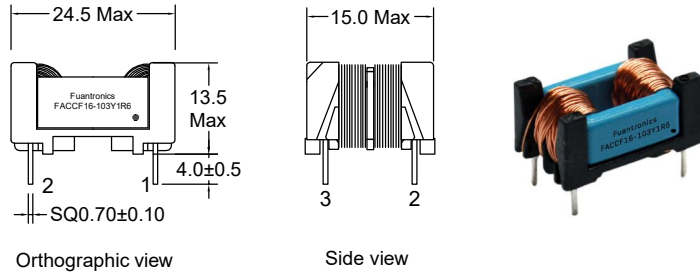
Orthographic view
