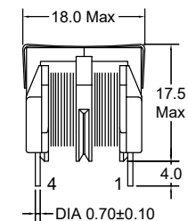
Orthographic view
