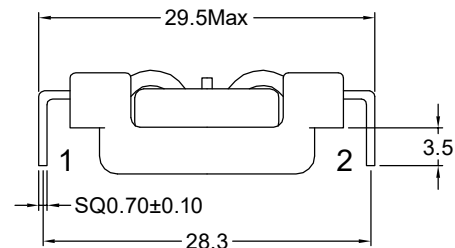
Orthographic view
