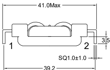
Orthographic view
